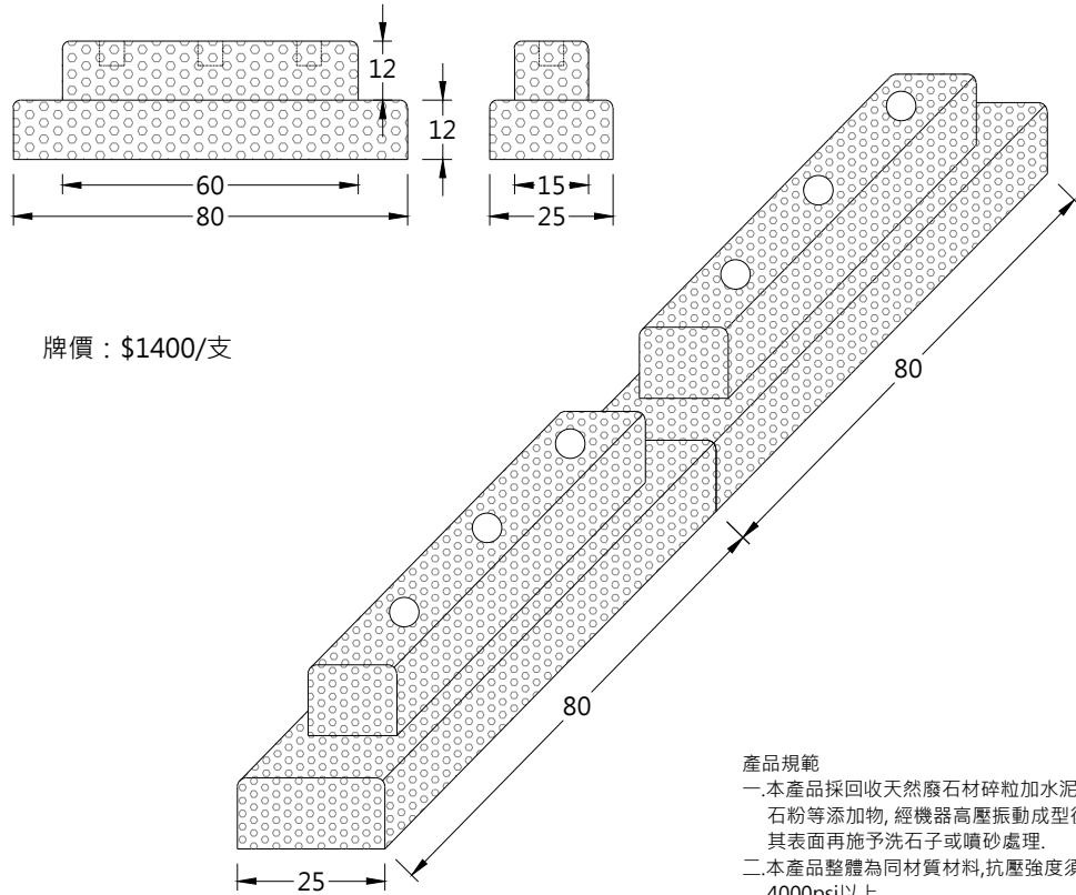
Q20 預鑄洗石子(噴砂)車止塊
