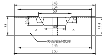
復育駁坎石 TYPE B 規格:150x100x35cm(±1cm) 牌價:$10700/M2
