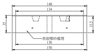
駁坎石 TYPE B 規格:150x100x35cm(±1cm) 牌價:$10700/M2
